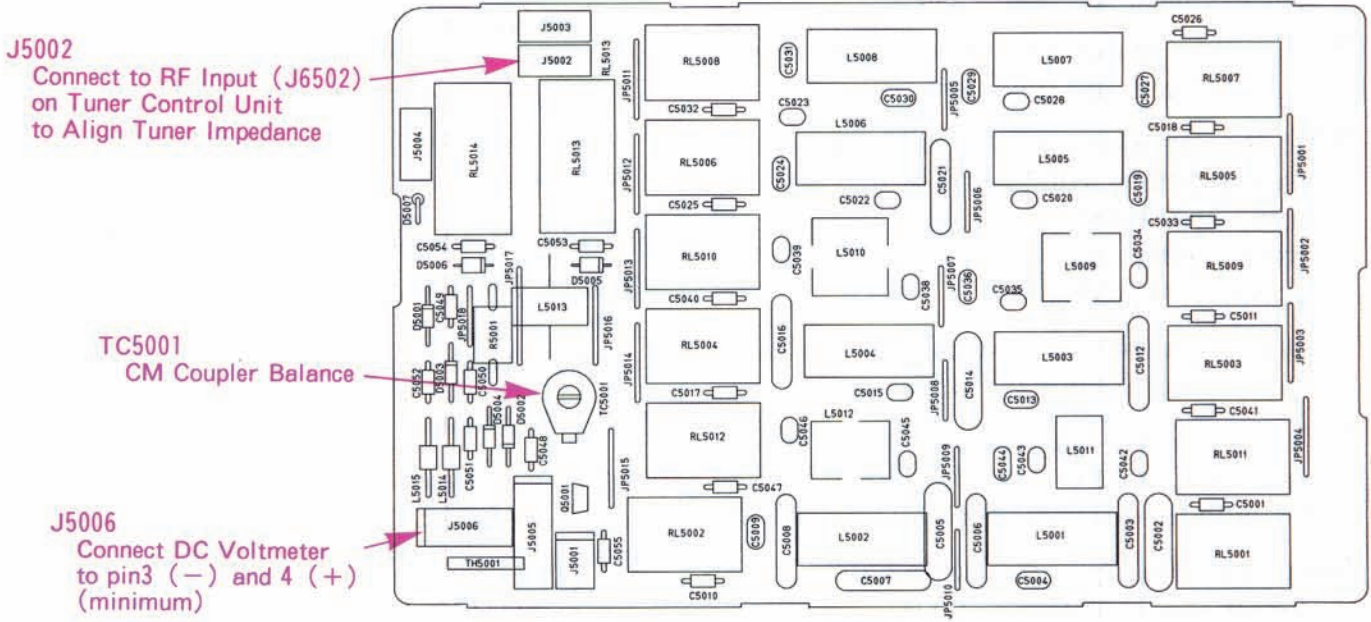
LPF Unit Test & Alignment Points
