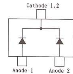
HSM2838 (A6) (D6508)
